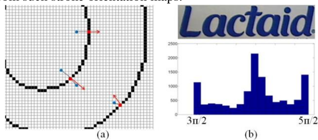
Fig. 8. (a) An example of stroke orientation label. The pixels denoted by blue points are assigned the gradient orientations (red arrows) at their nearest edge pixels, denoted by the red points. (b) A 210 \times 54 text patch and its 16-bin histogram of quantized stroke orientations.
